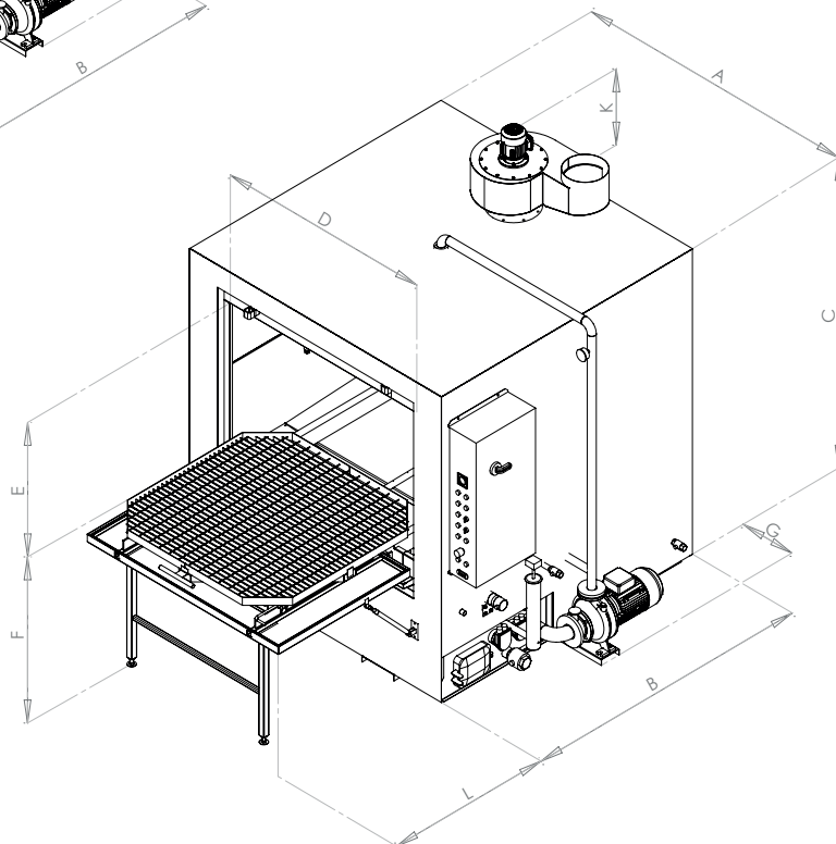
Cleaning machine with hinged door C-800SS-KD...C-1600SS-KD
